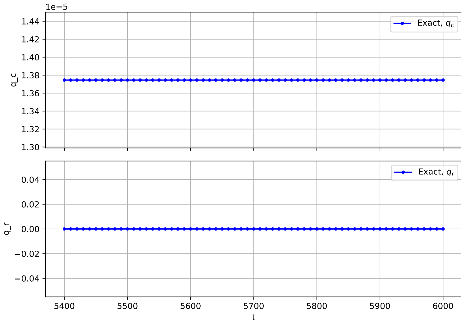
Trajectory No. 3171
