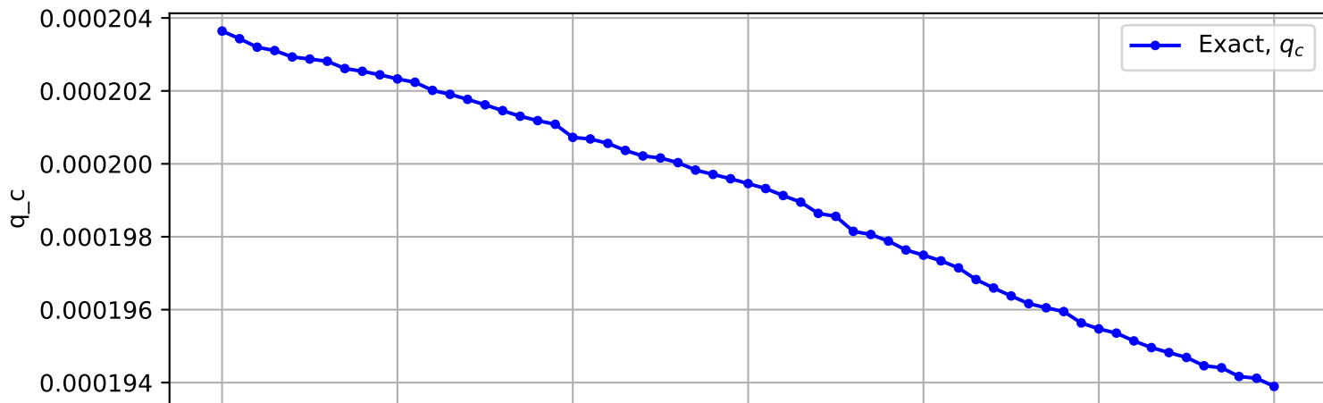
Trajectory No. 3179
