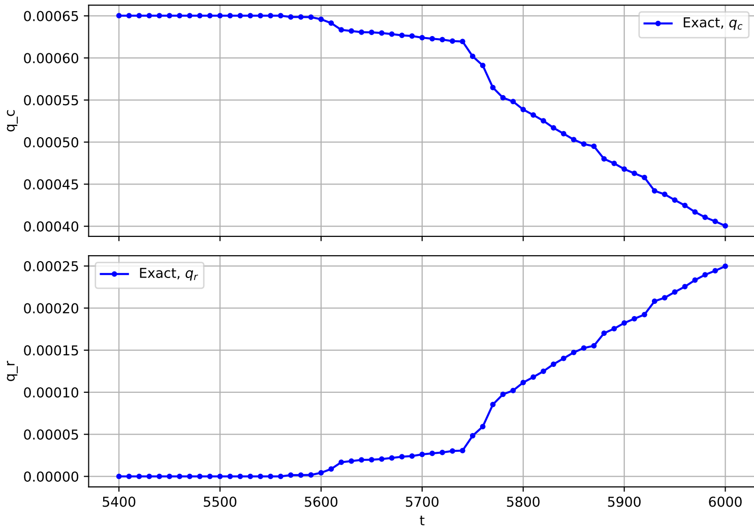
Trajectory No. 319
