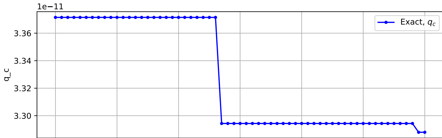
Trajectory No. 3192
