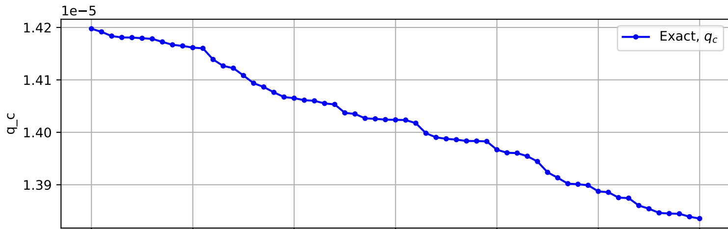
Trajectory No. 3195
