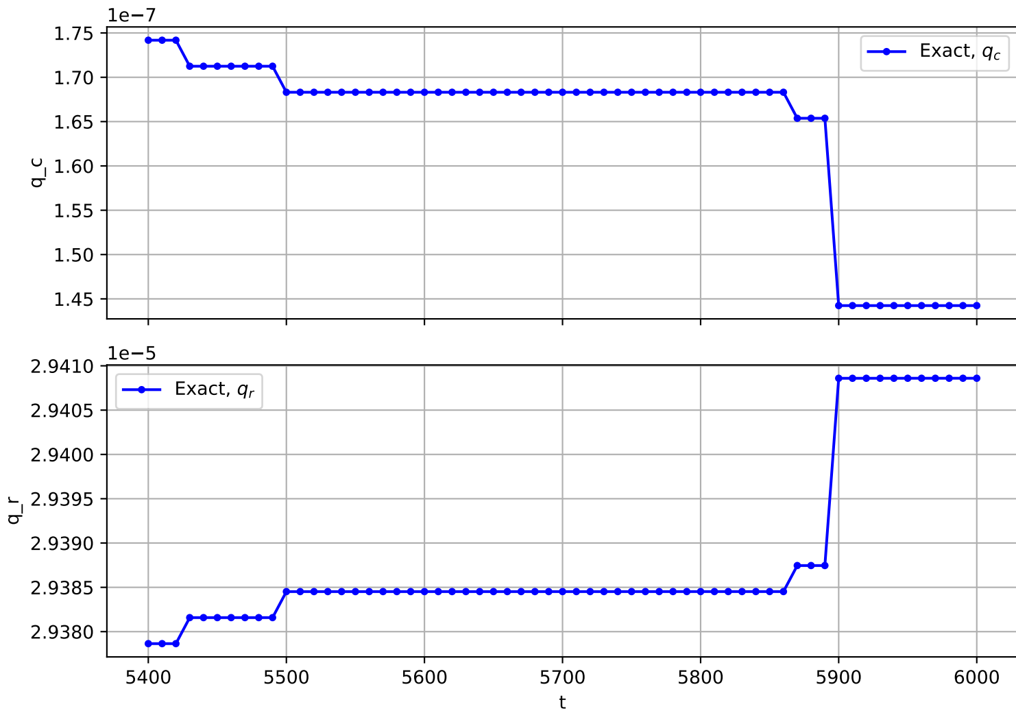
Trajectory No. 3250
