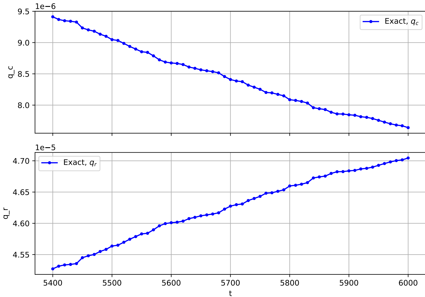
Trajectory No. 3259
