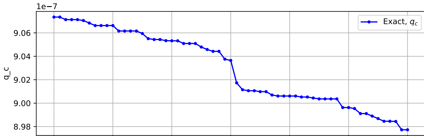
Trajectory No. 3308
