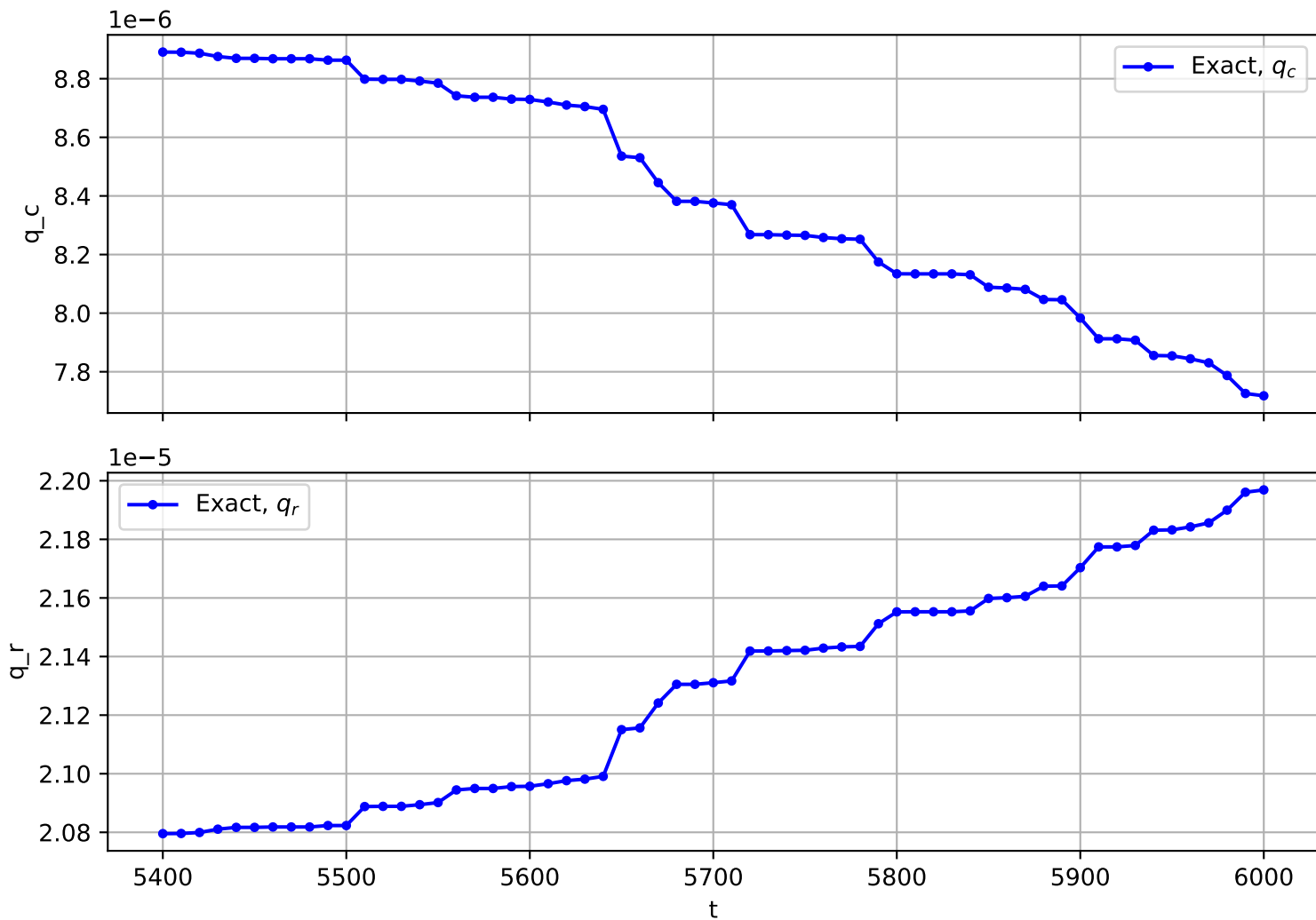
Trajectory No. 347
