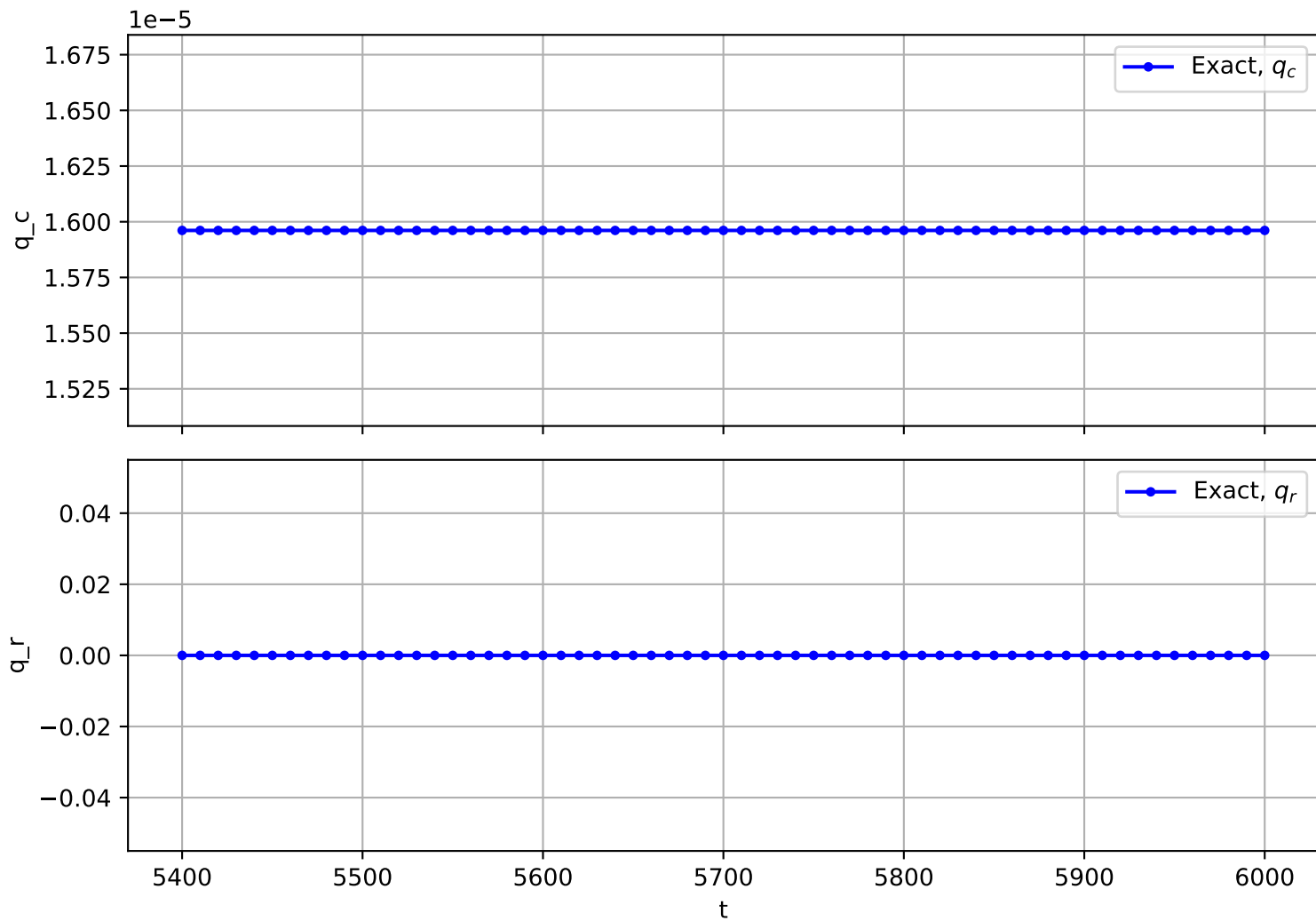
Trajectory No. 3481
