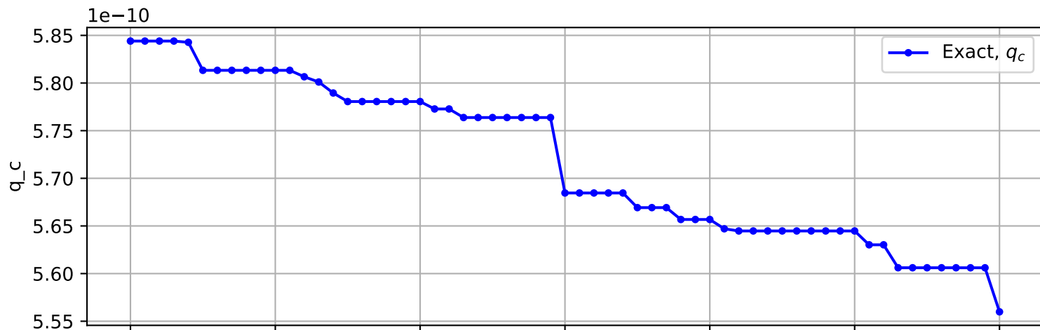
Trajectory No. 353
