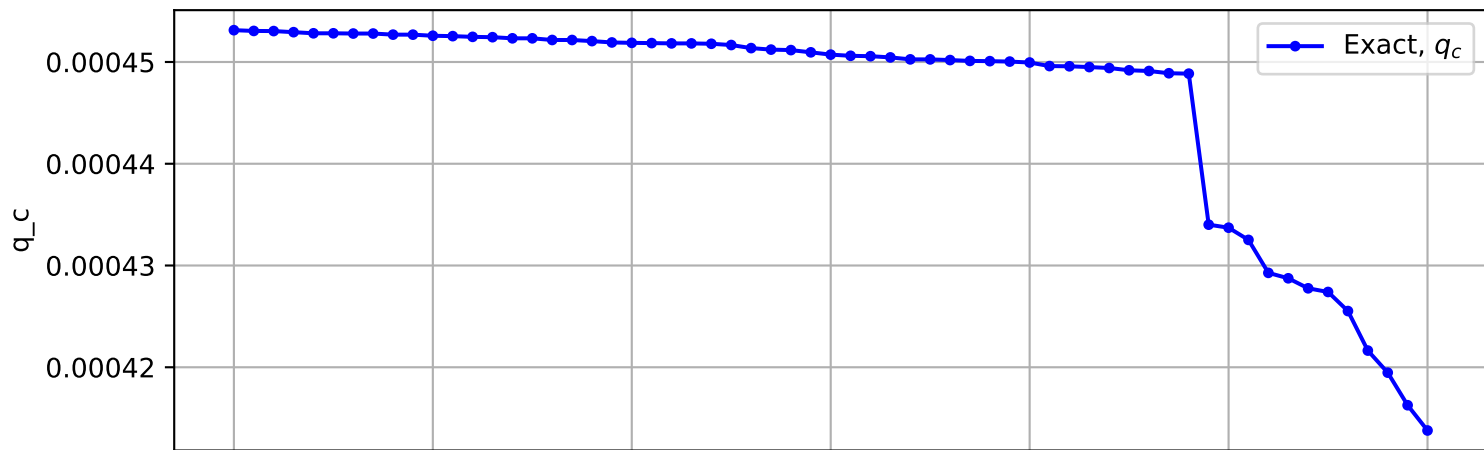
Trajectory No. 370
