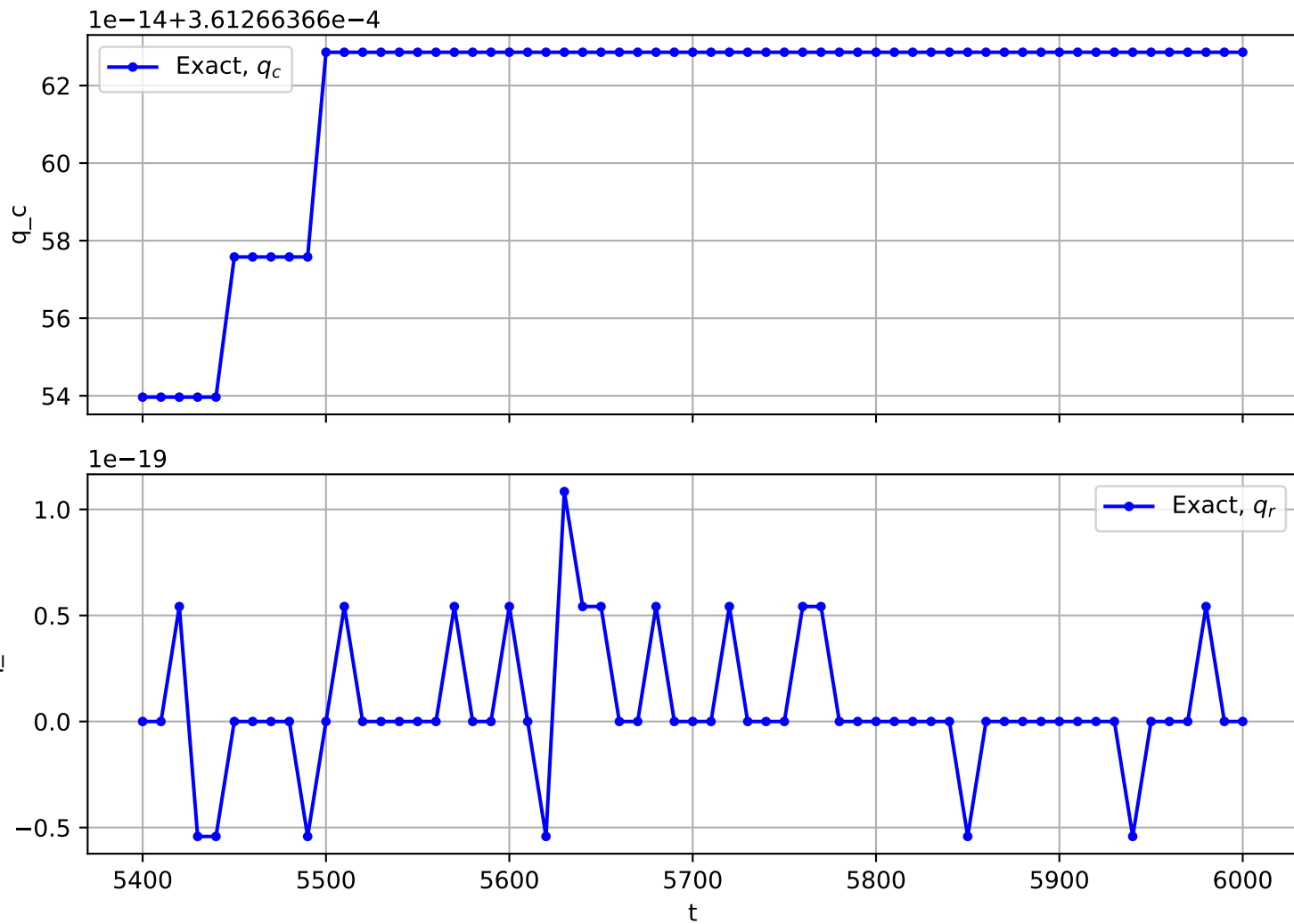
Trajectory No. 396
