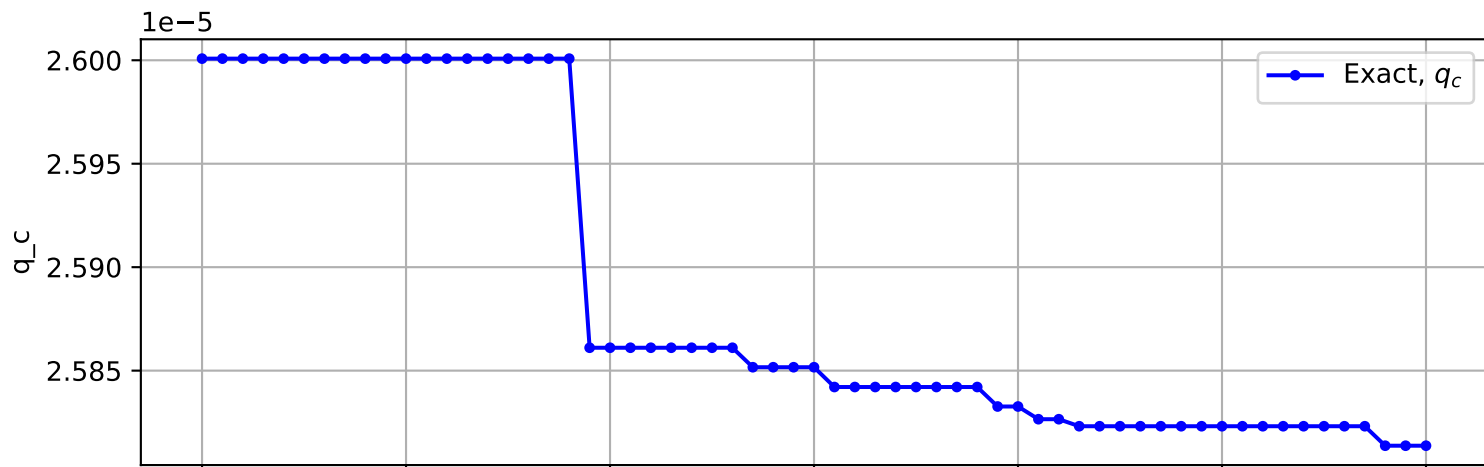
Trajectory No. 436
