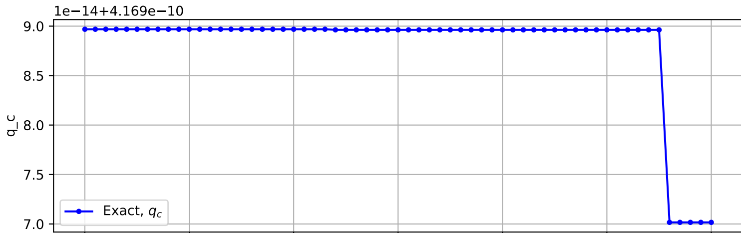
Trajectory No. 438
