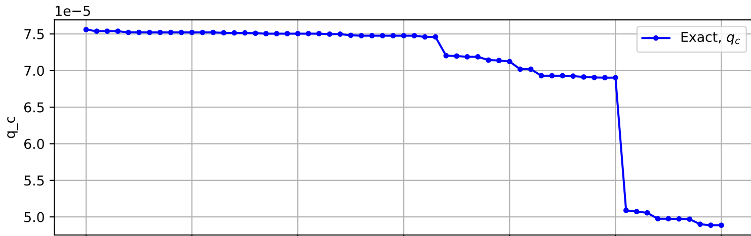
Trajectory No. 476
