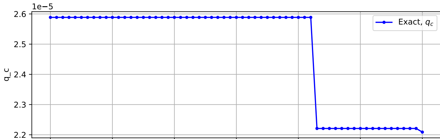
Trajectory No. 481
