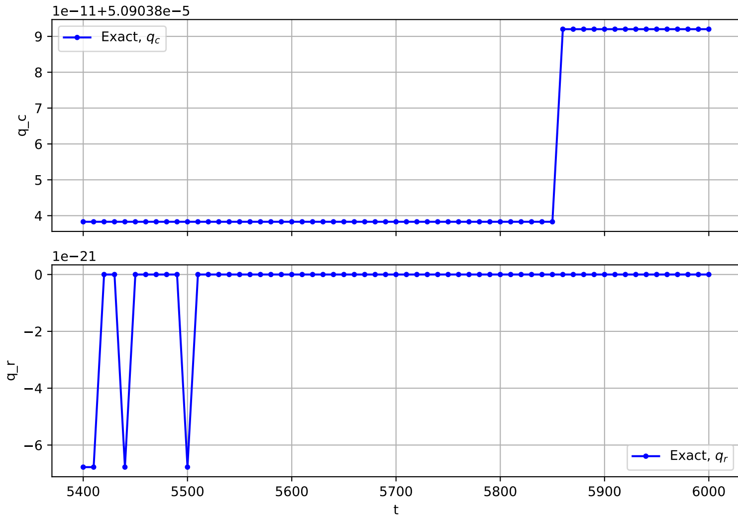
Trajectory No. 489
