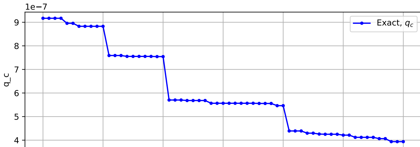
Trajectory No. 534
