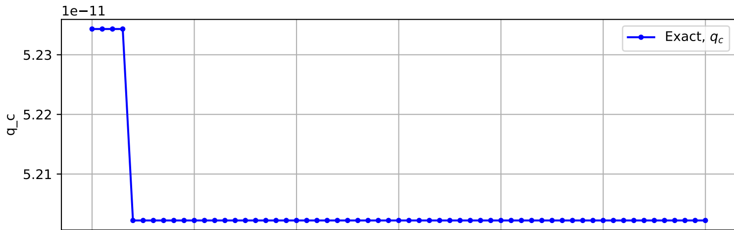
Trajectory No. 550
