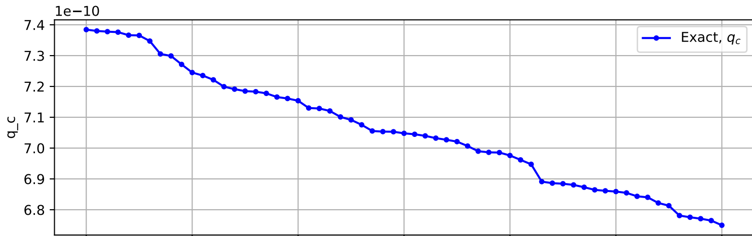
Trajectory No. 567
