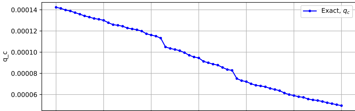
Trajectory No. 62
