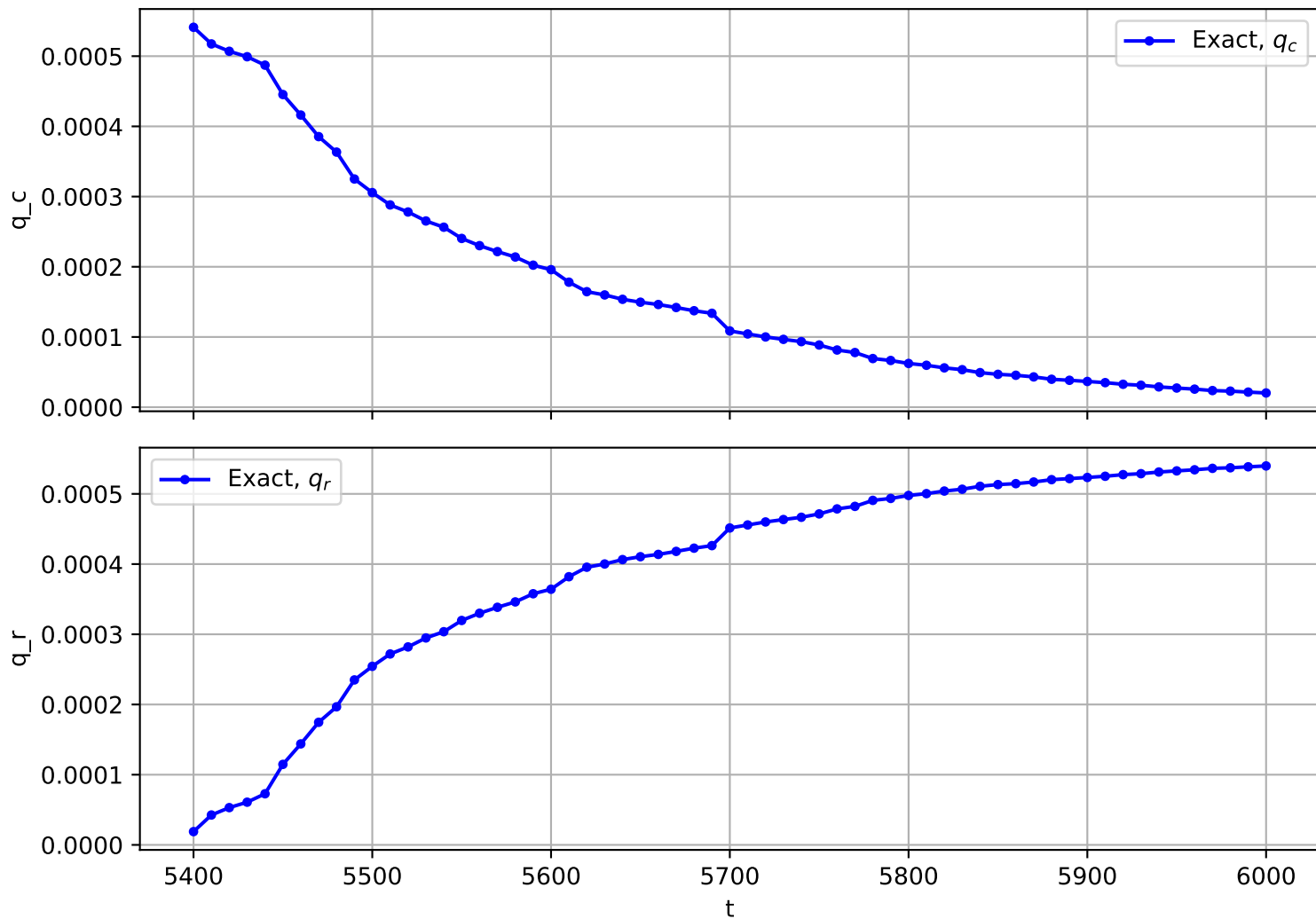
Trajectory No. 647
