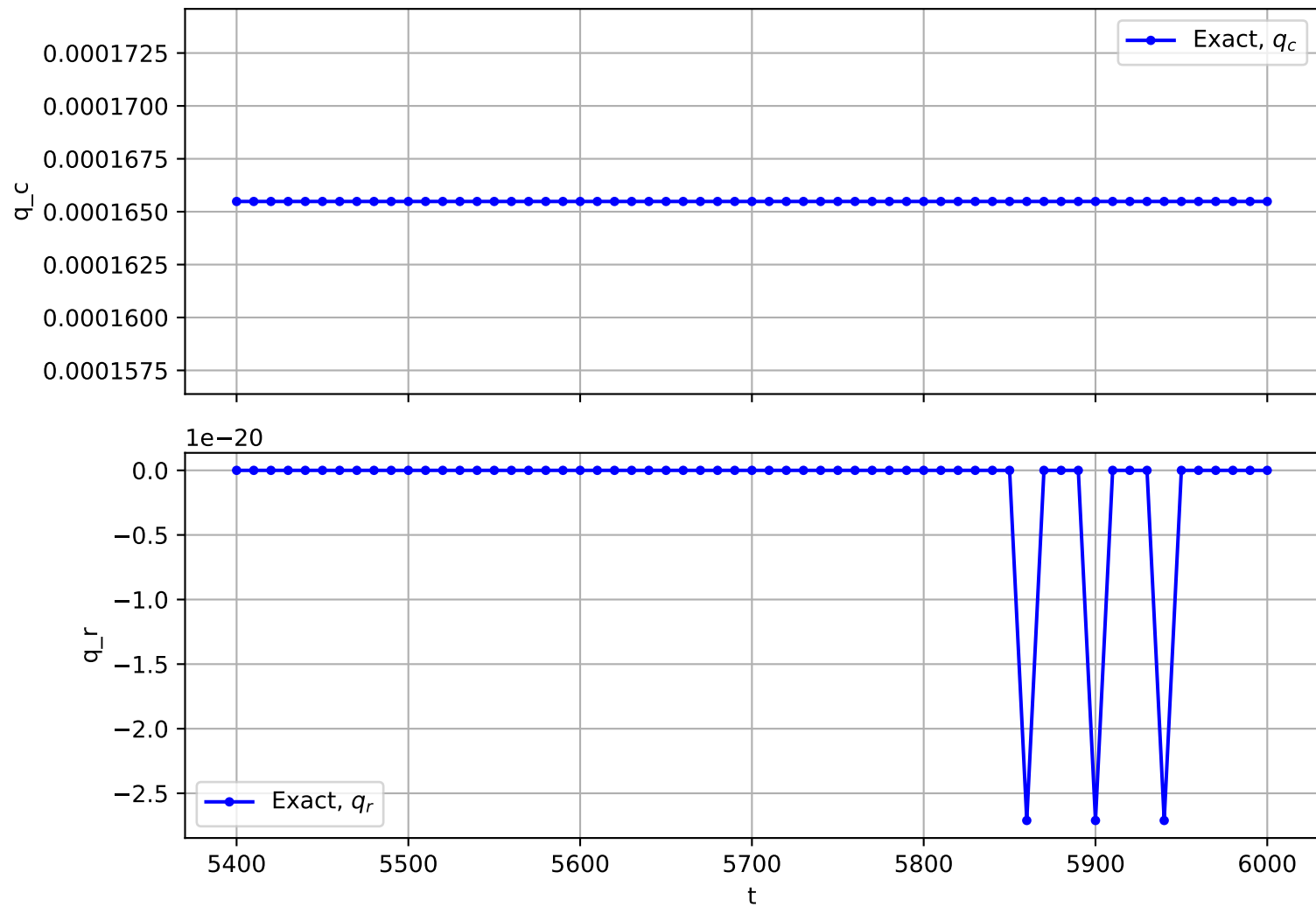
Trajectory No. 648
