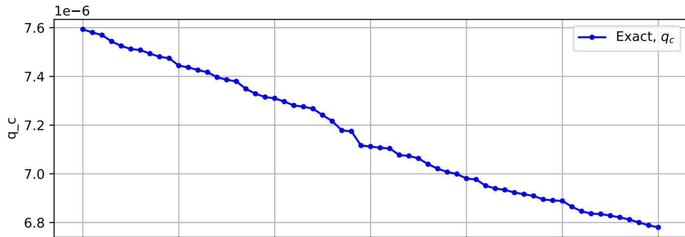
Trajectory No. 684
