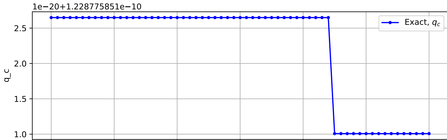
Trajectory No. 70
