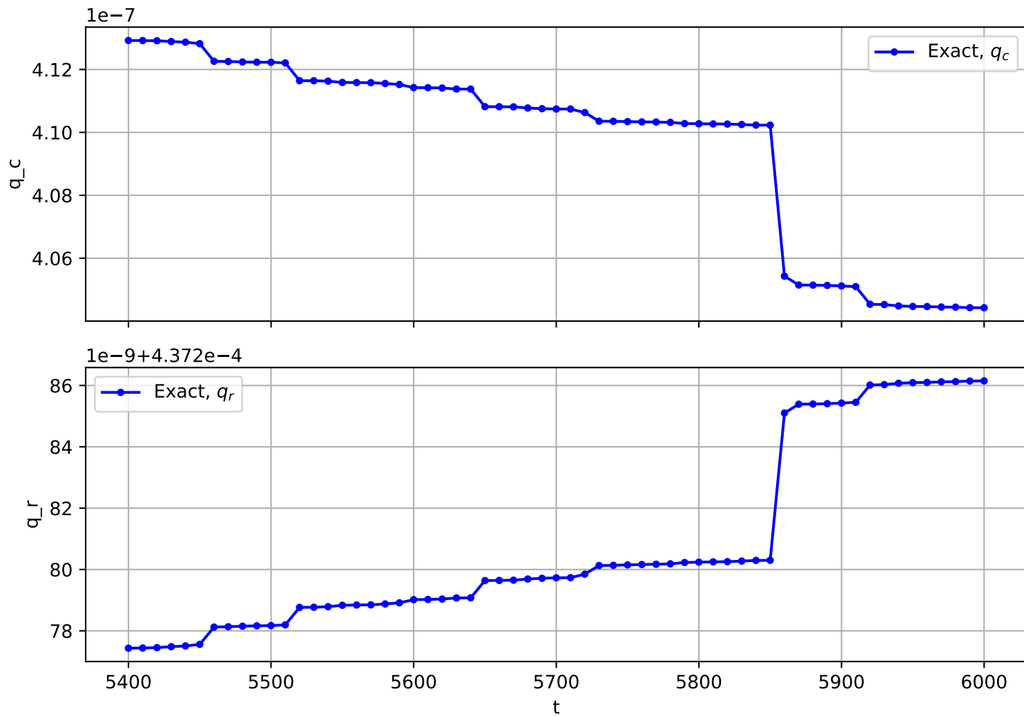
Trajectory No. 726
