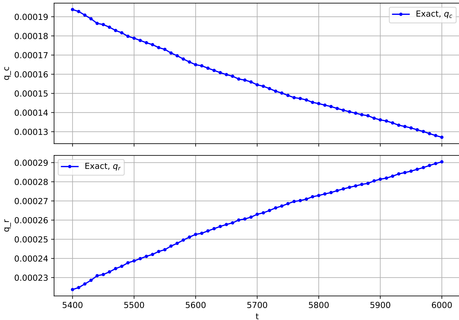
Trajectory No. 745
