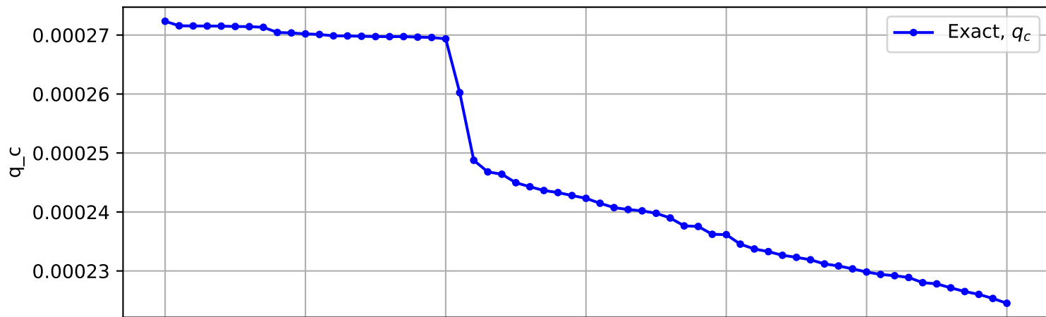
Trajectory No. 797
