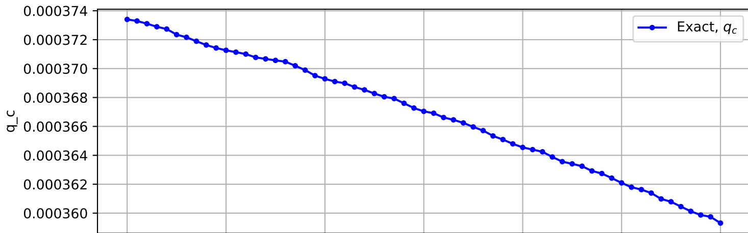
Trajectory No. 827
