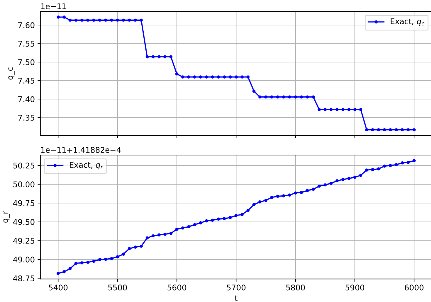
Trajectory No. 860
