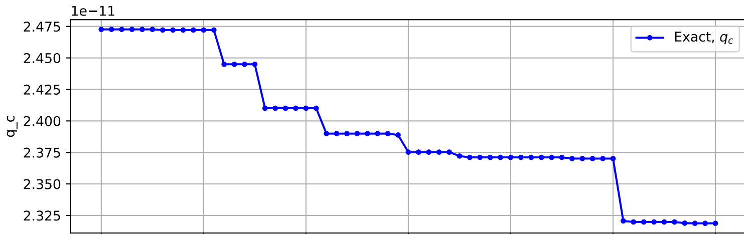
Trajectory No. 911
