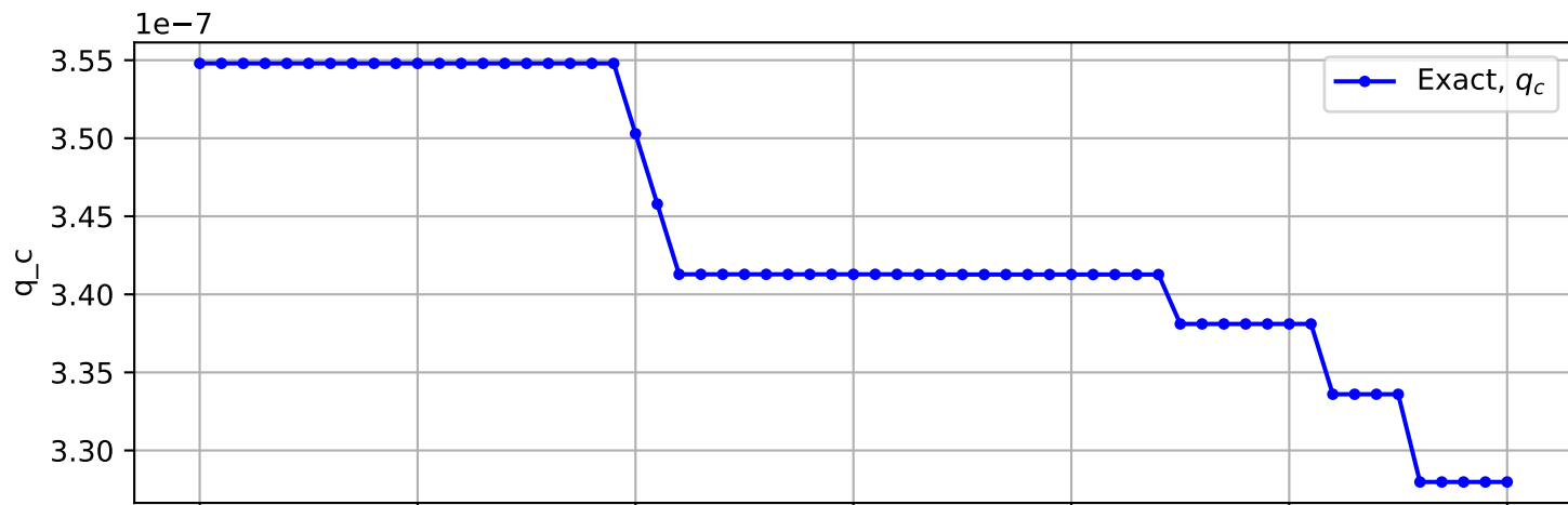
Trajectory No. 924
