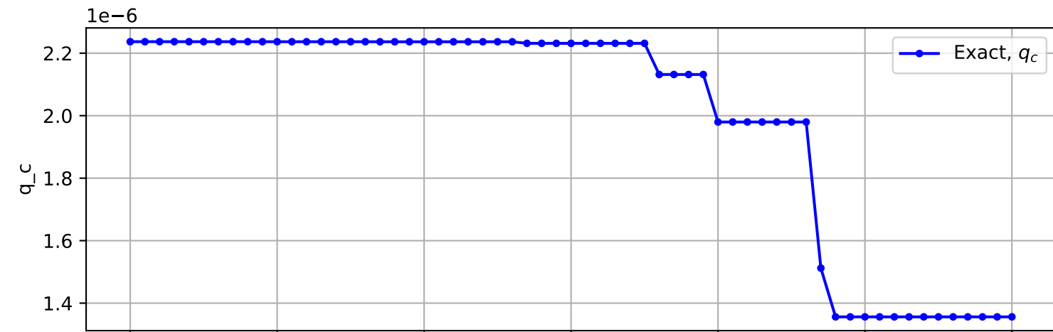
Trajectory No. 931
