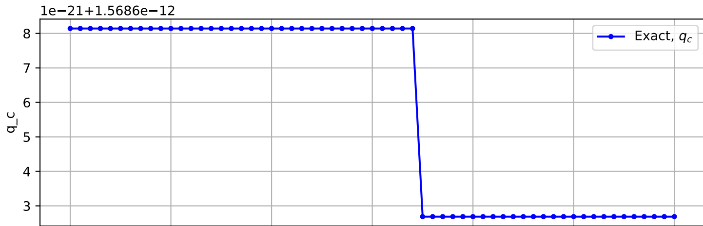
Trajectory No. 932
