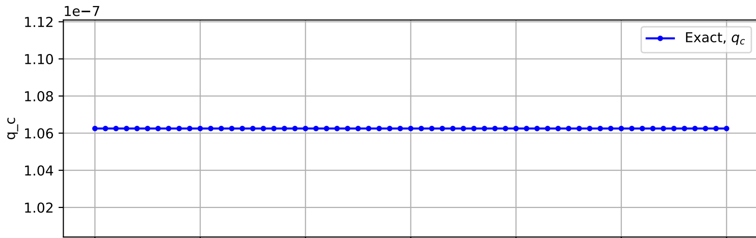
Trajectory No. 942
