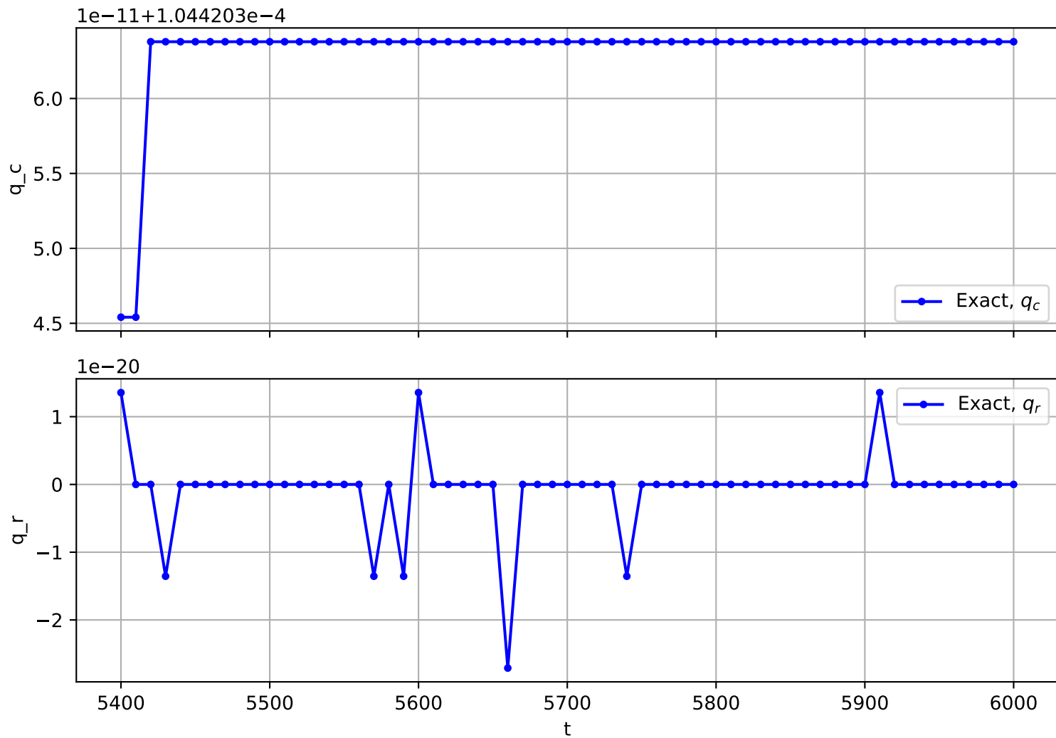
Trajectory No. 95
