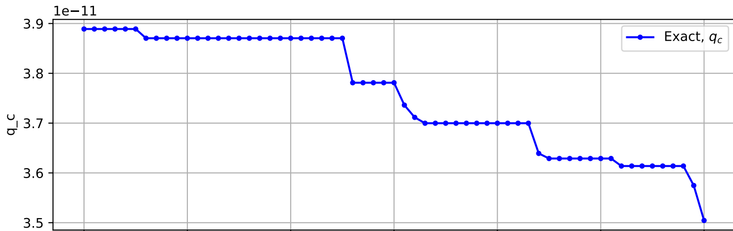
Trajectory No. 952
