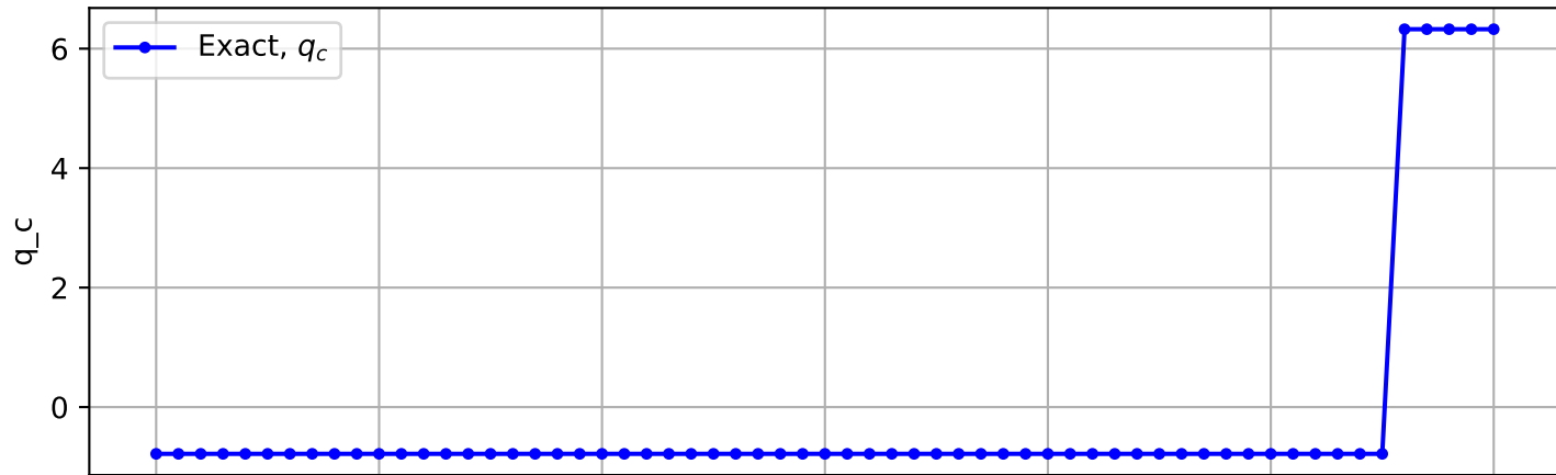
Trajectory No. 963
