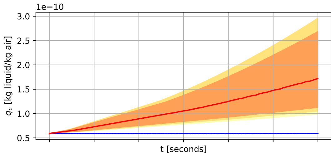
Trajectory No. 1000
