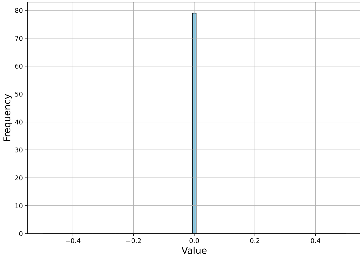
Variable 0, feature 8: x_1^3
