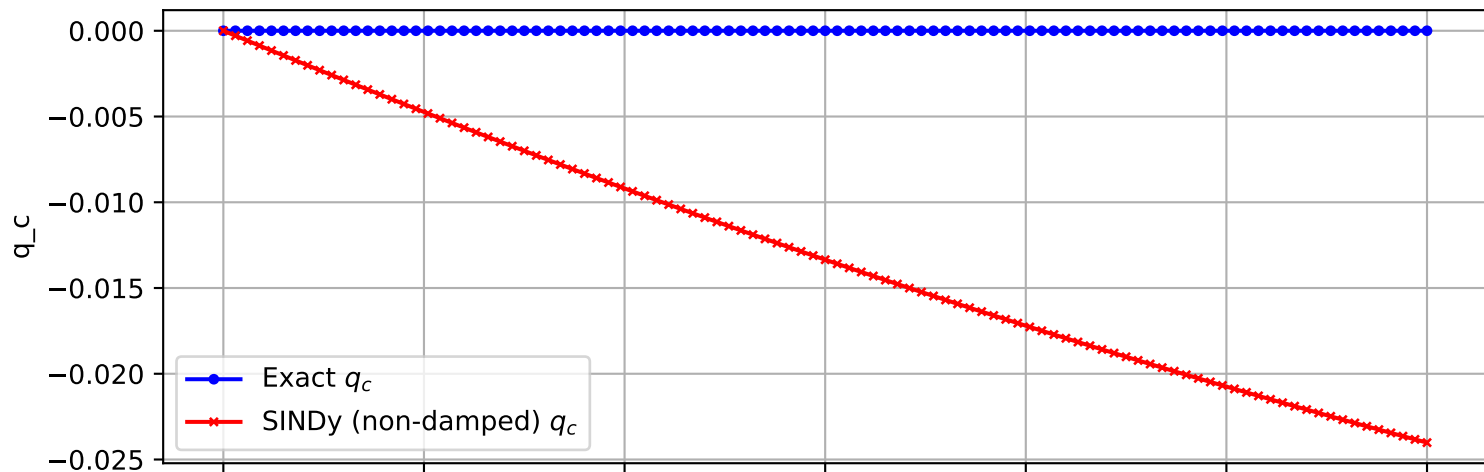
Trajectory 1000 (non-damped)
