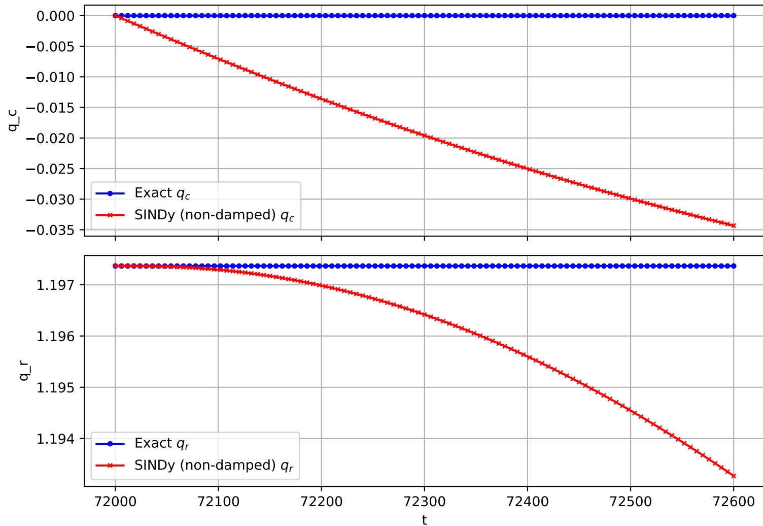
Trajectory 1003 (non-damped)
