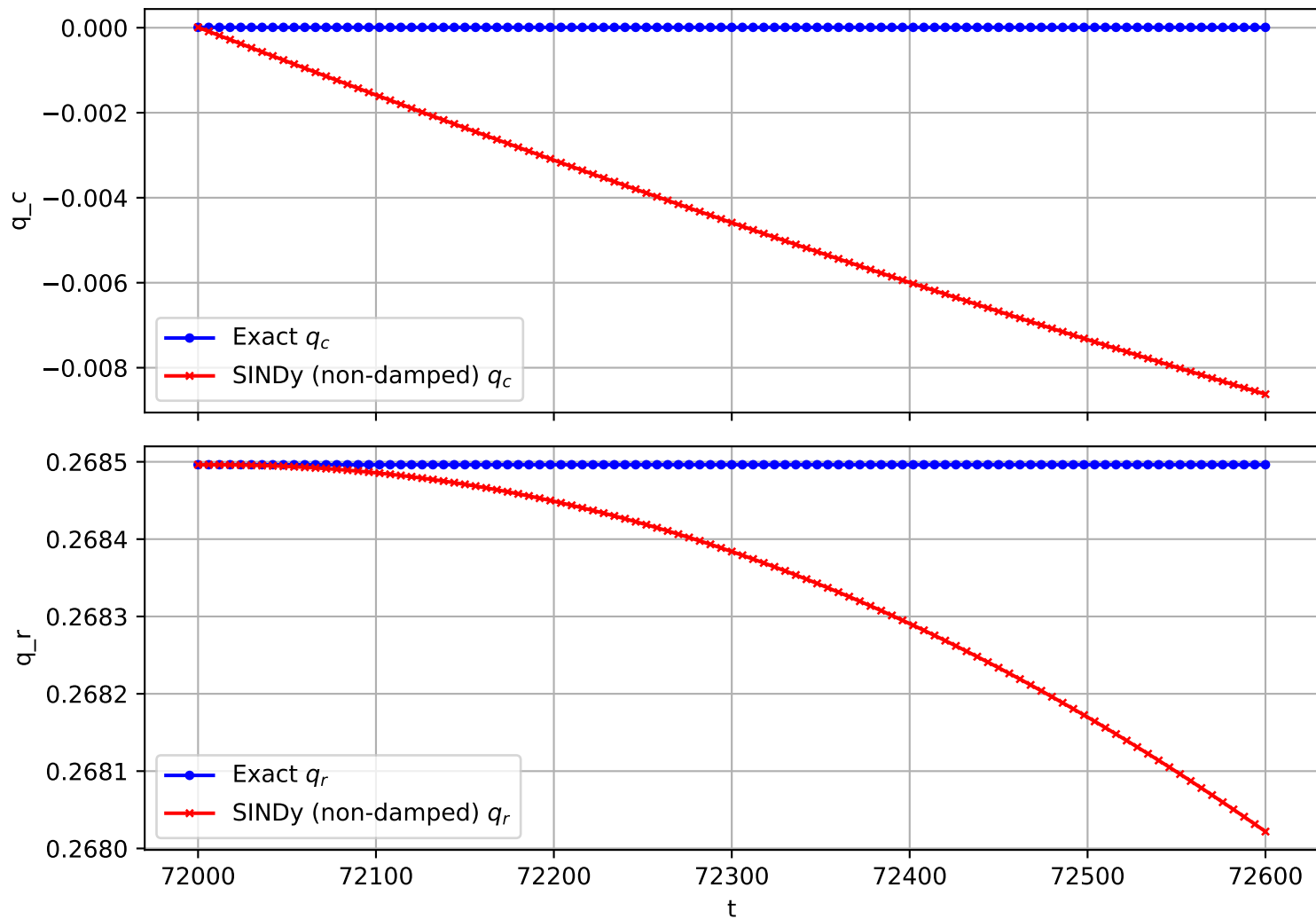
Trajectory 1007 (non-damped)
