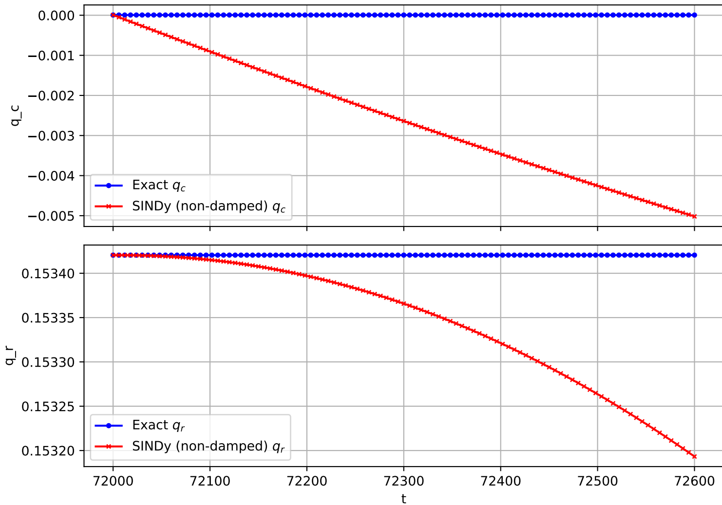
Trajectory 1008 (non-damped)
