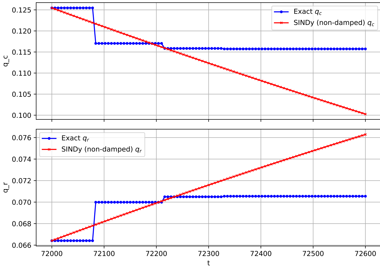
Trajectory 101 (non-damped)
