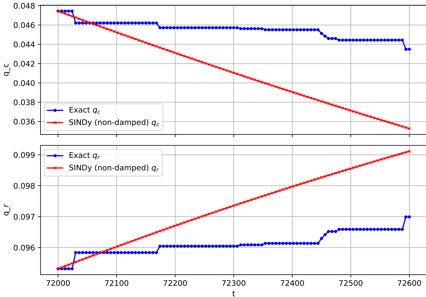
Trajectory 1012 (non-damped)
