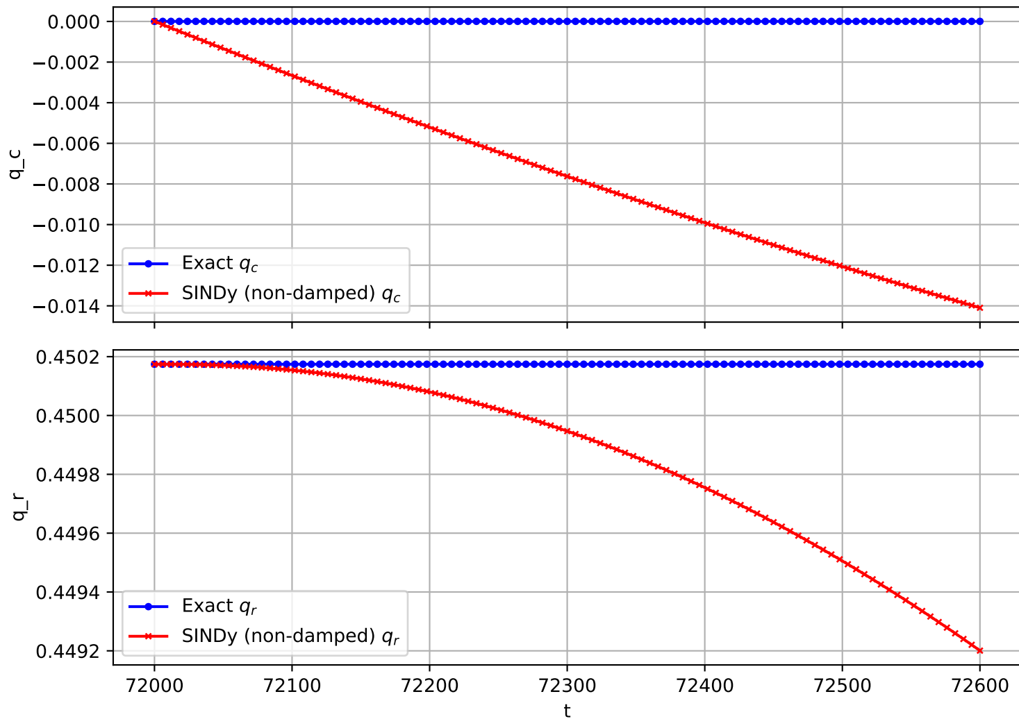
Trajectory 1024 (non-damped)
