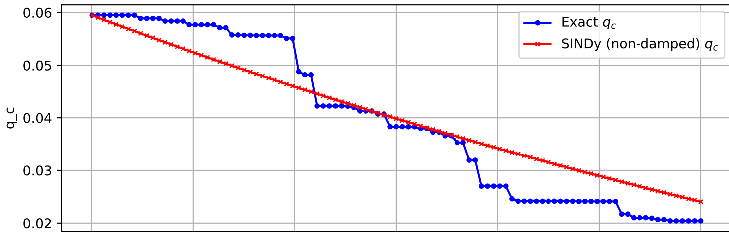
Trajectory 1031 (non-damped)
