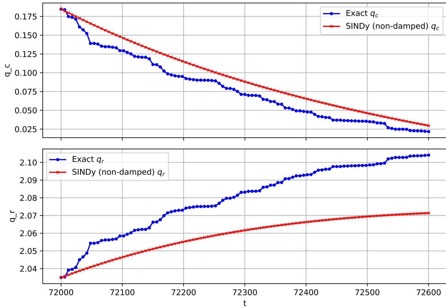
Trajectory 1032 (non-damped)
